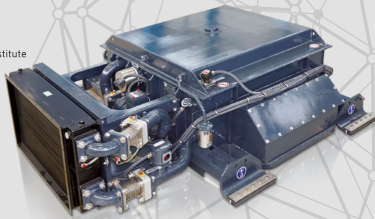
TRANSFORMER FOR EMU Tested on shock & vibrations at ISMES/CESI Institute in Italy Type: MOZ 1510-27,5, Croatia Rated power: 1510/4x275/160/100/150kVA Rated voltage: 25000/4x800/1000/400/340V
