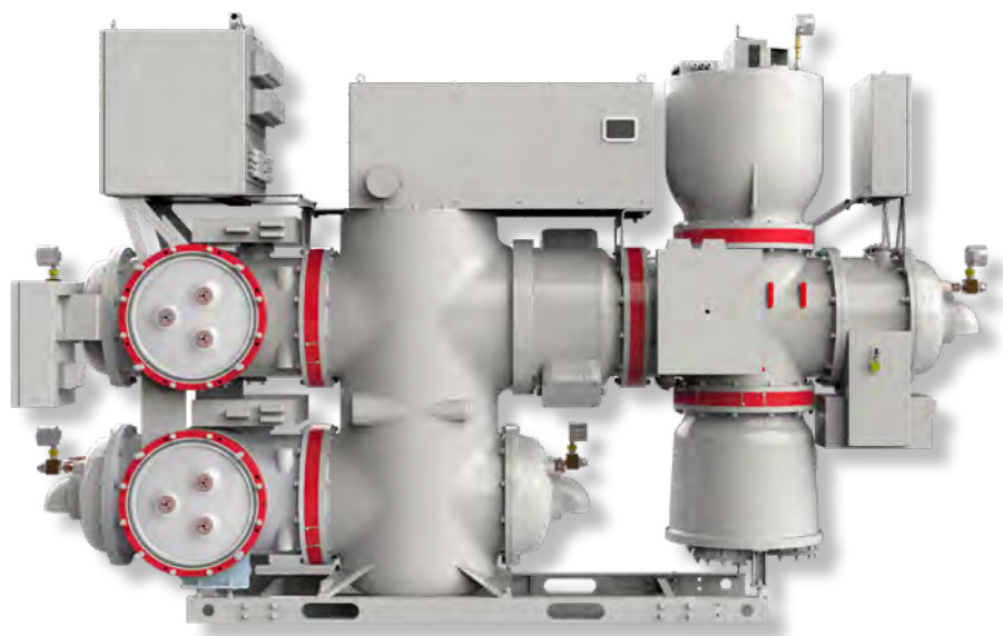
Metal-enclosed gas-insulated switchgear, rated voltage up to 145 kV, type K8D.6-N
