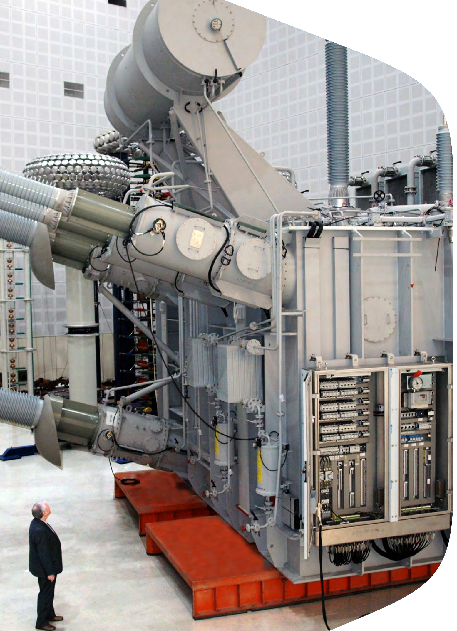
HVDC converter transformer delivered to New Zealand
